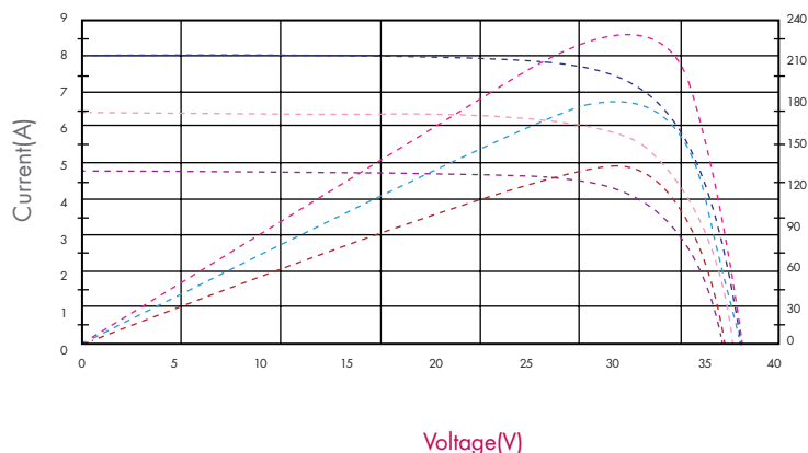
Characteristics Module IV Graph 230W
